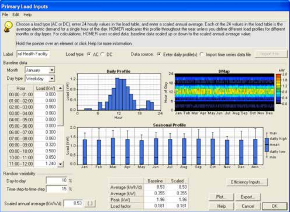
Fig. A3. Baseline data with daily noise of 10% and hourly noise of 15%
